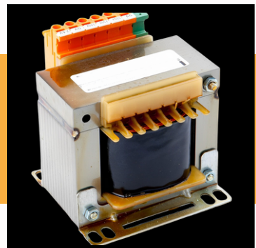
Isolation Transformer with Earth Screen between Primary and Secondary
