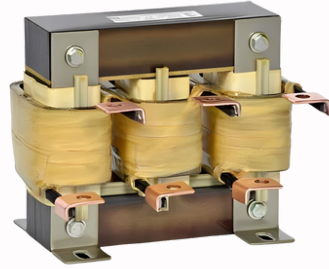
Line Reactor, 3-Ph, Core and Coil, 3%, 480V, 50HP
